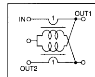
Directional coupler Fig. 4
