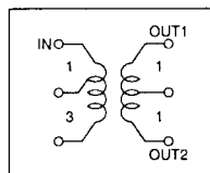
Distributor Fig. 3
