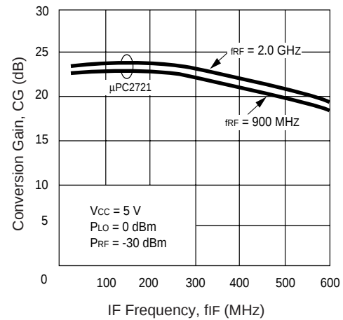
UPC2721 CONVERSION GAIN vs. IF FREQUENCY
