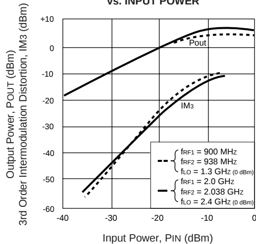
UPC2721 IM3 AND OUTPUT POWER vs. INPUT POWER
